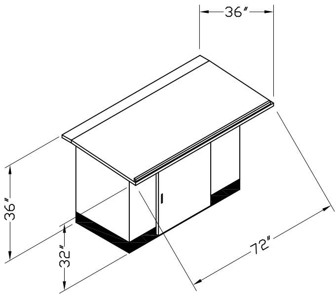
PLAN TABLE WITH STORAGE
