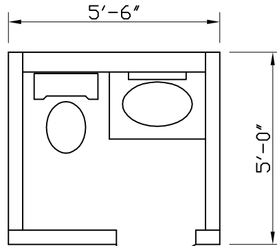
(OPTION #1) HALF BATH
