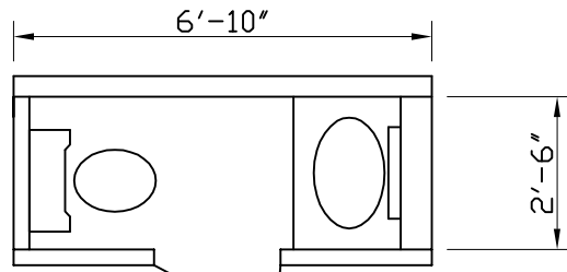
(OPTION #1) HALF BATH
